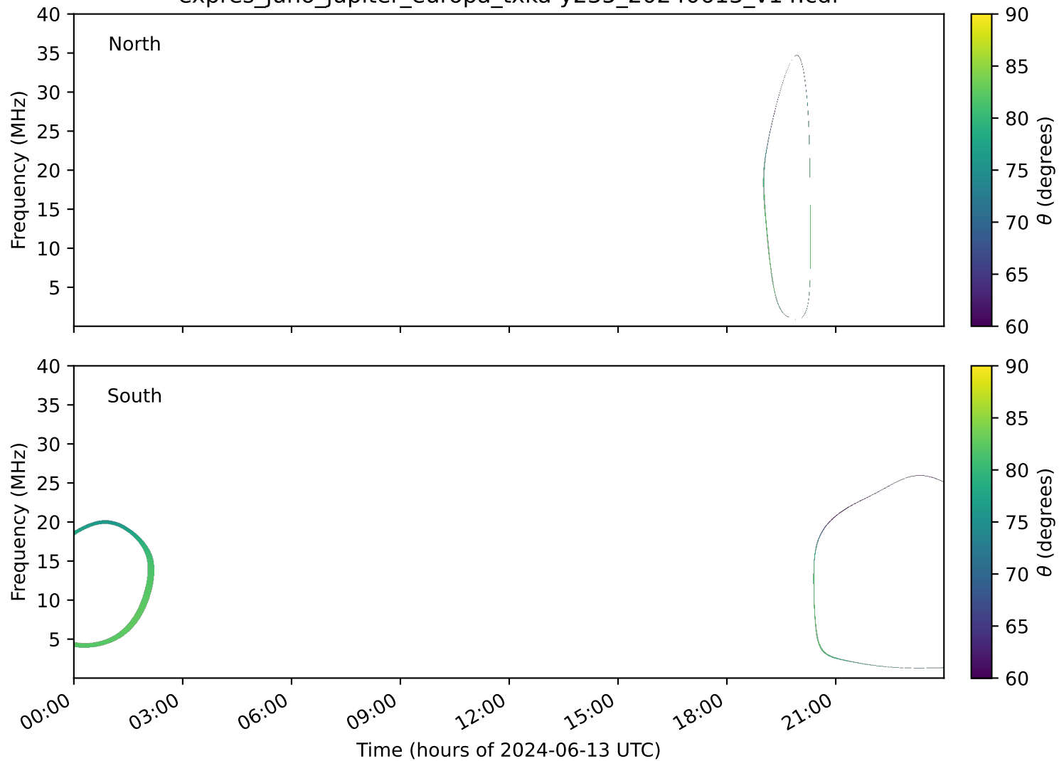
expres_juno_jupiter_europa_txka-y235_20240613_v14.cdf
