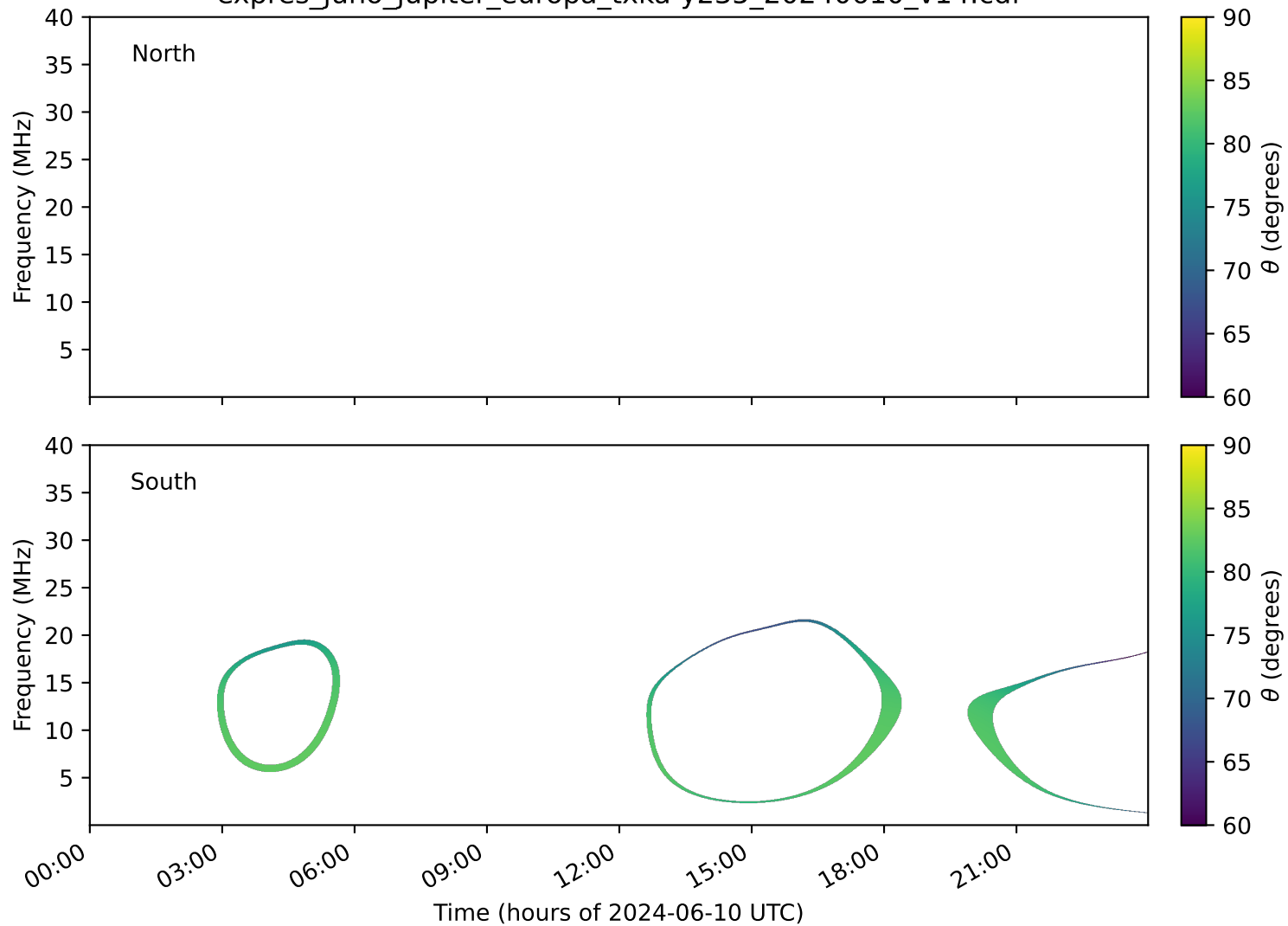
expres_juno_jupiter_europa_txka-y235_20240610_v14.cdf
