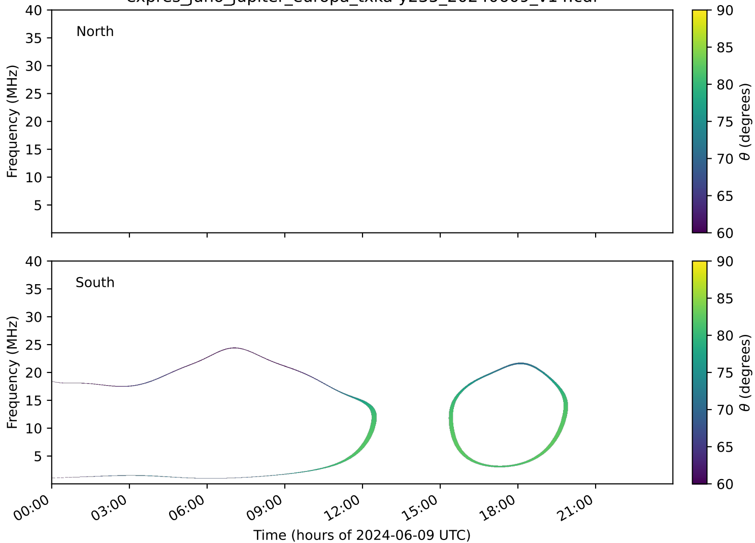
expres_juno_jupiter_europa_txka-y235_20240609_v14.cdf
