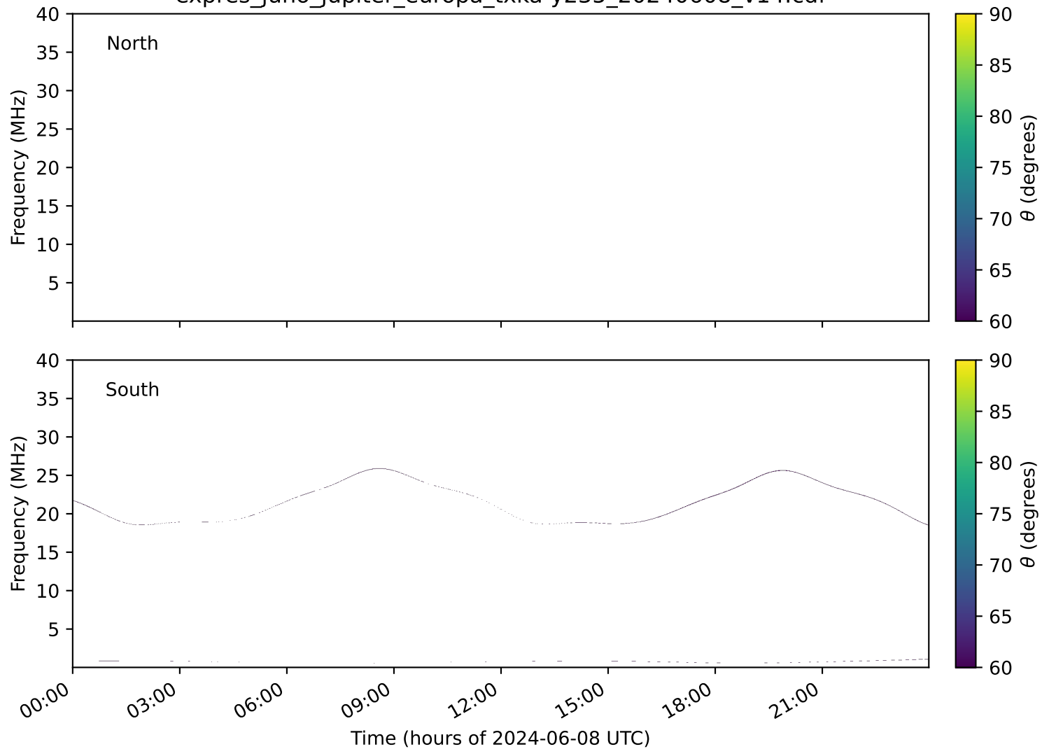
expres_juno_jupiter_europa_txka-y235_20240608_v14.cdf
