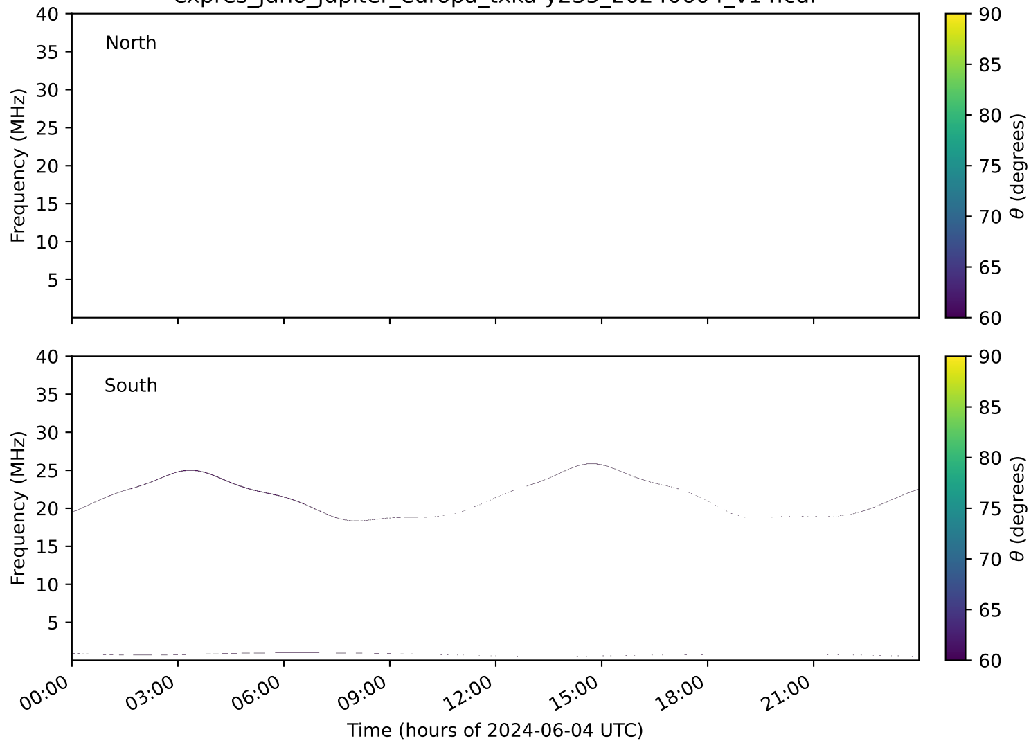
expres_juno_jupiter_europa_txka-y235_20240604_v14.cdf
