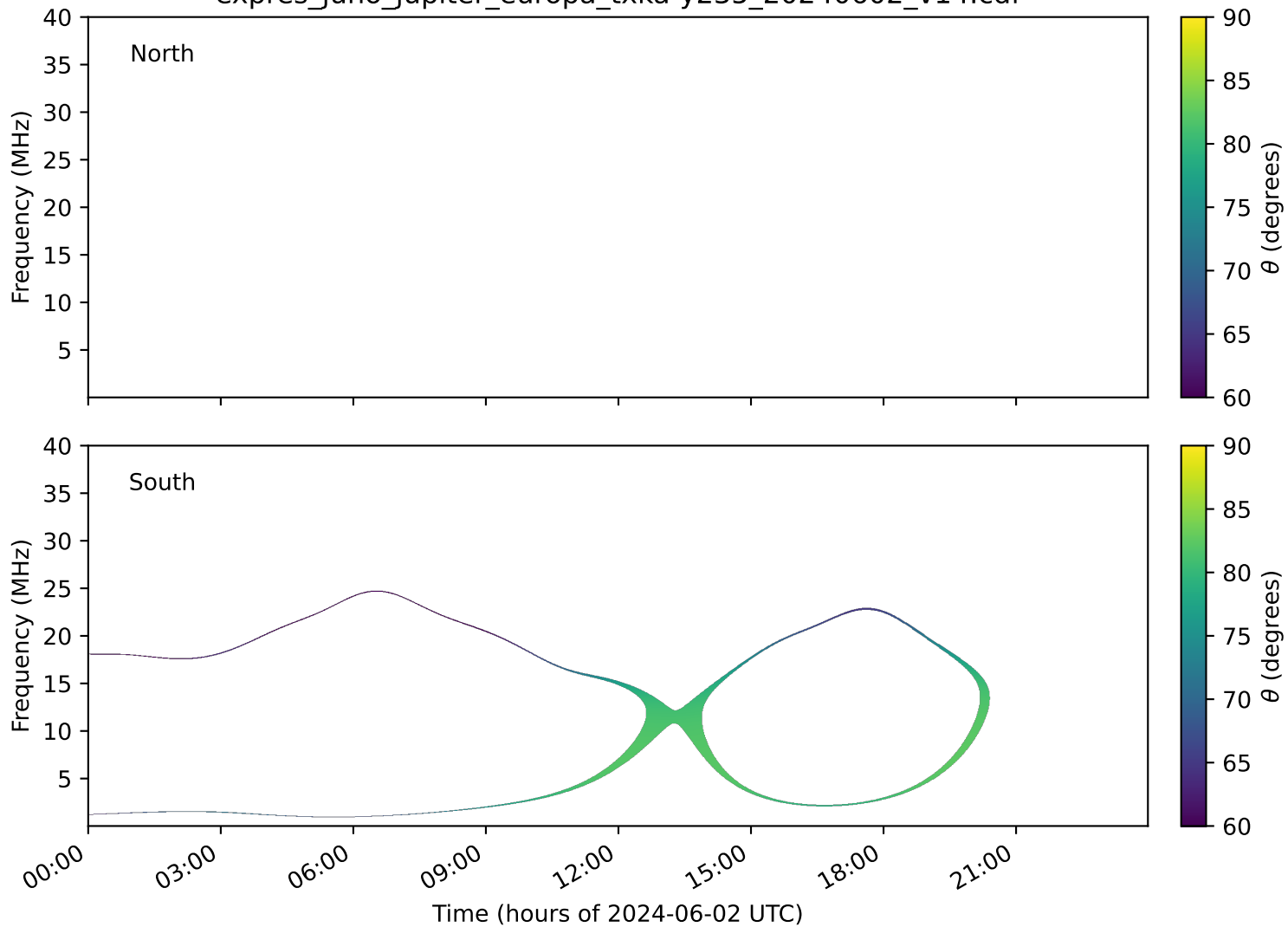
expres_juno_jupiter_europa_txka-y235_20240602_v14.cdf
