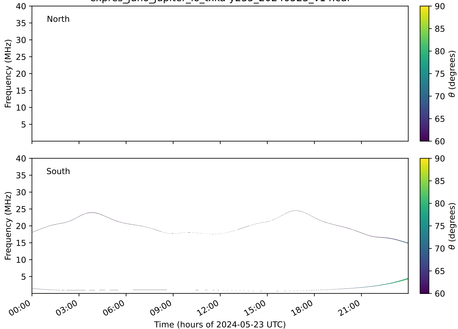
expres_juno_jupiter_io_txka-y235_20240523_v14.cdf
