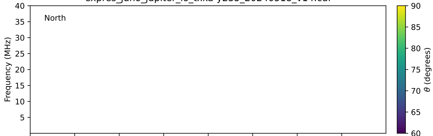
expres_juno_jupiter_io_txka-y235_20240518_v14.cdf
