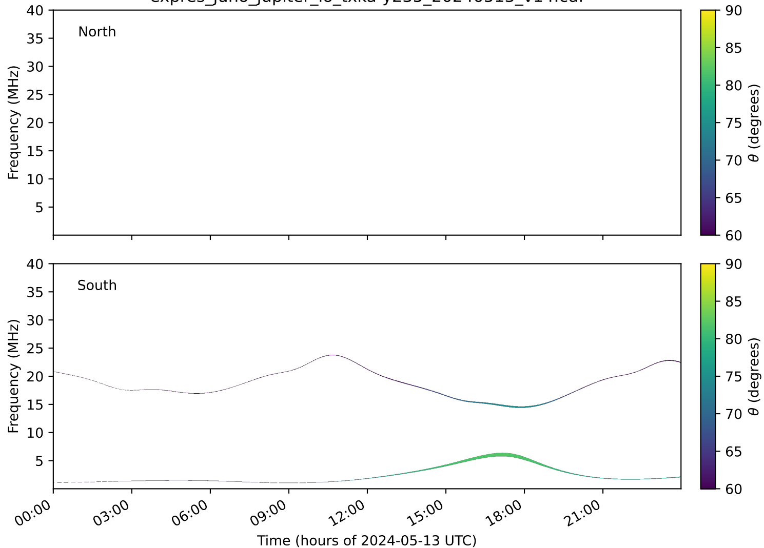
expres_juno_jupiter_io_txka-y235_20240513_v14.cdf
