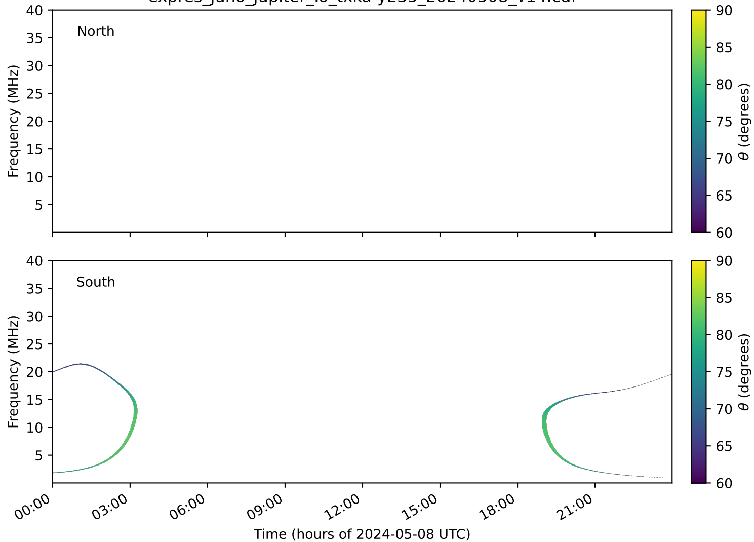
expres_juno_jupiter_io_txka-y235_20240508_v14.cdf
