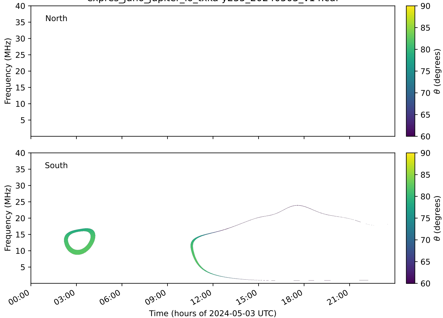
expres_juno_jupiter_io_txka-y235_20240503_v14.cdf
