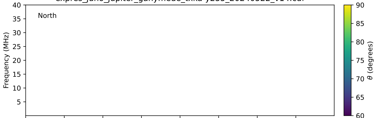
expres_juno_jupiter_ganymede_txka-y235_20240522_v14.cdf
