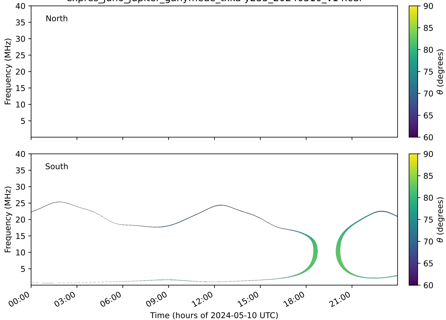
expres_juno_jupiter_ganymede_txka-y235_20240510_v14.cdf
