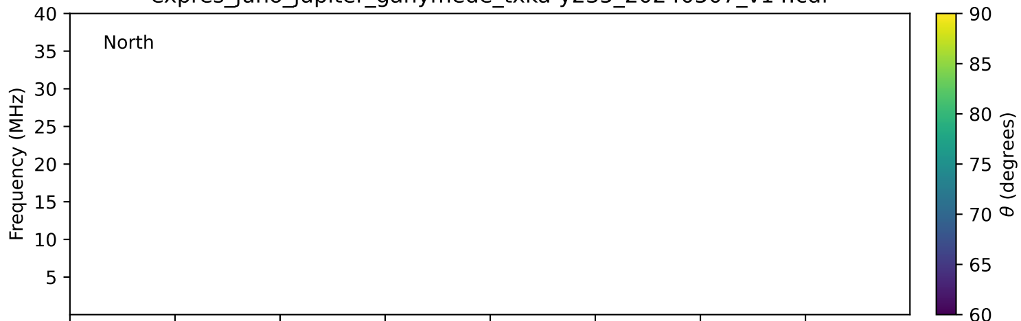
expres_juno_jupiter_ganymede_txka-y235_20240507_v14.cdf
