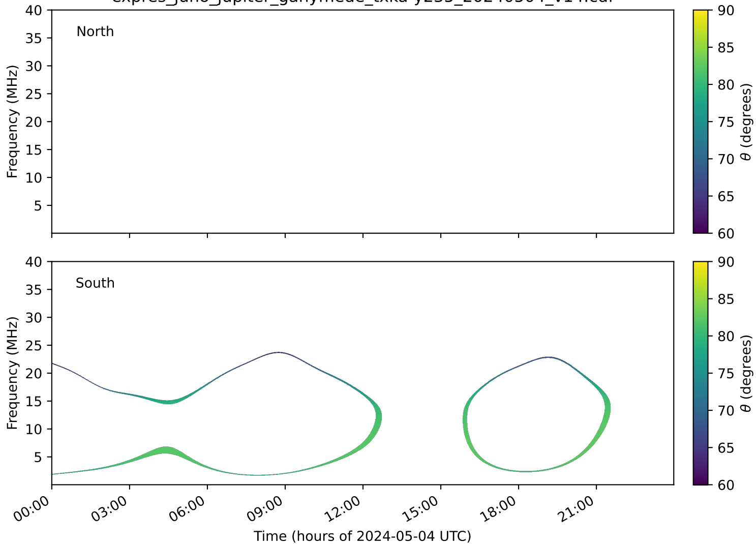
expres_juno_jupiter_ganymede_txka-y235_20240504_v14.cdf
