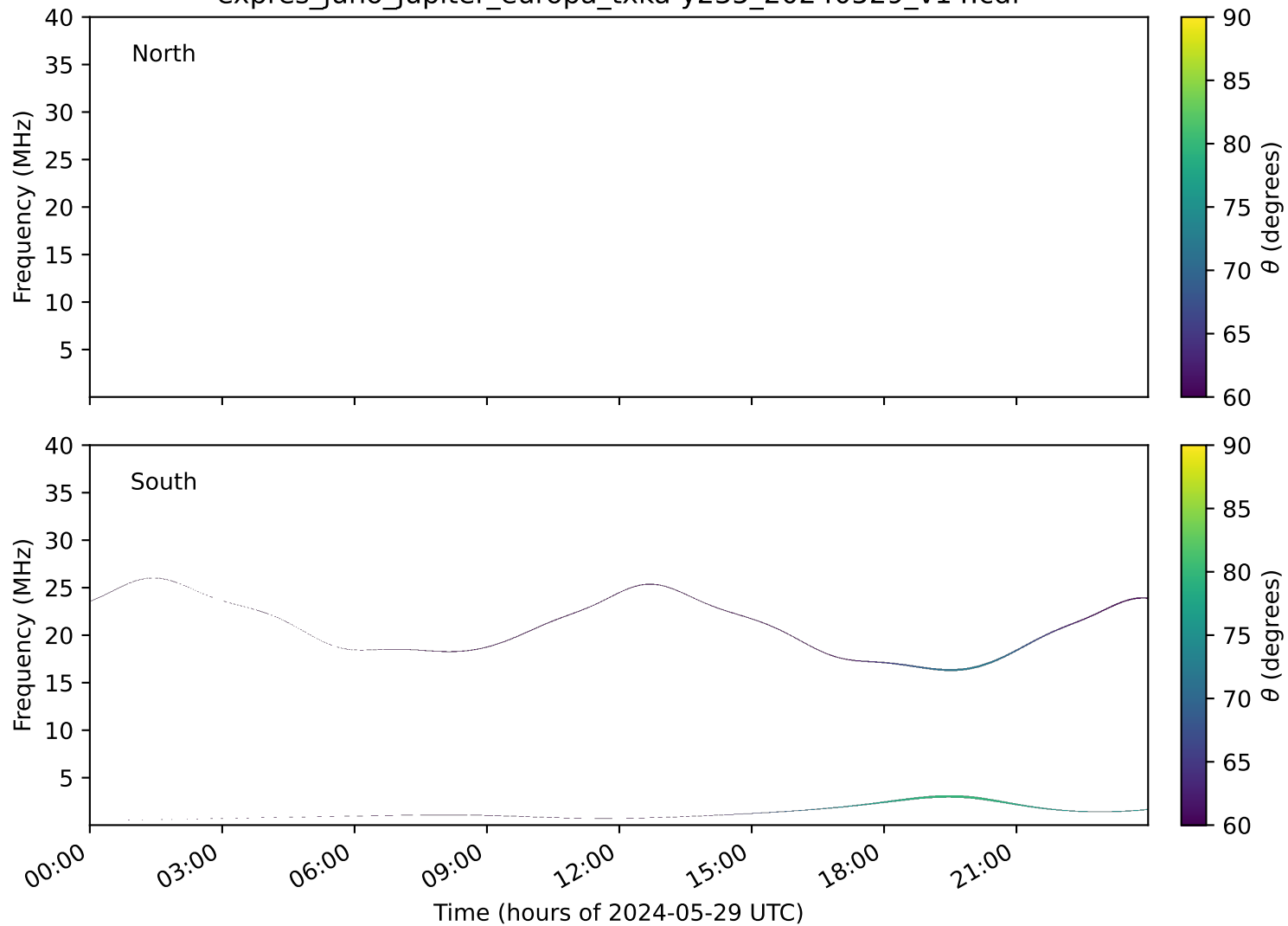
expres_juno_jupiter_europa_txka-y235_20240529_v14.cdf
