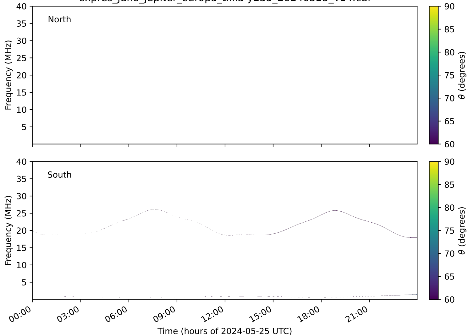
expres_juno_jupiter_europa_txka-y235_20240525_v14.cdf
