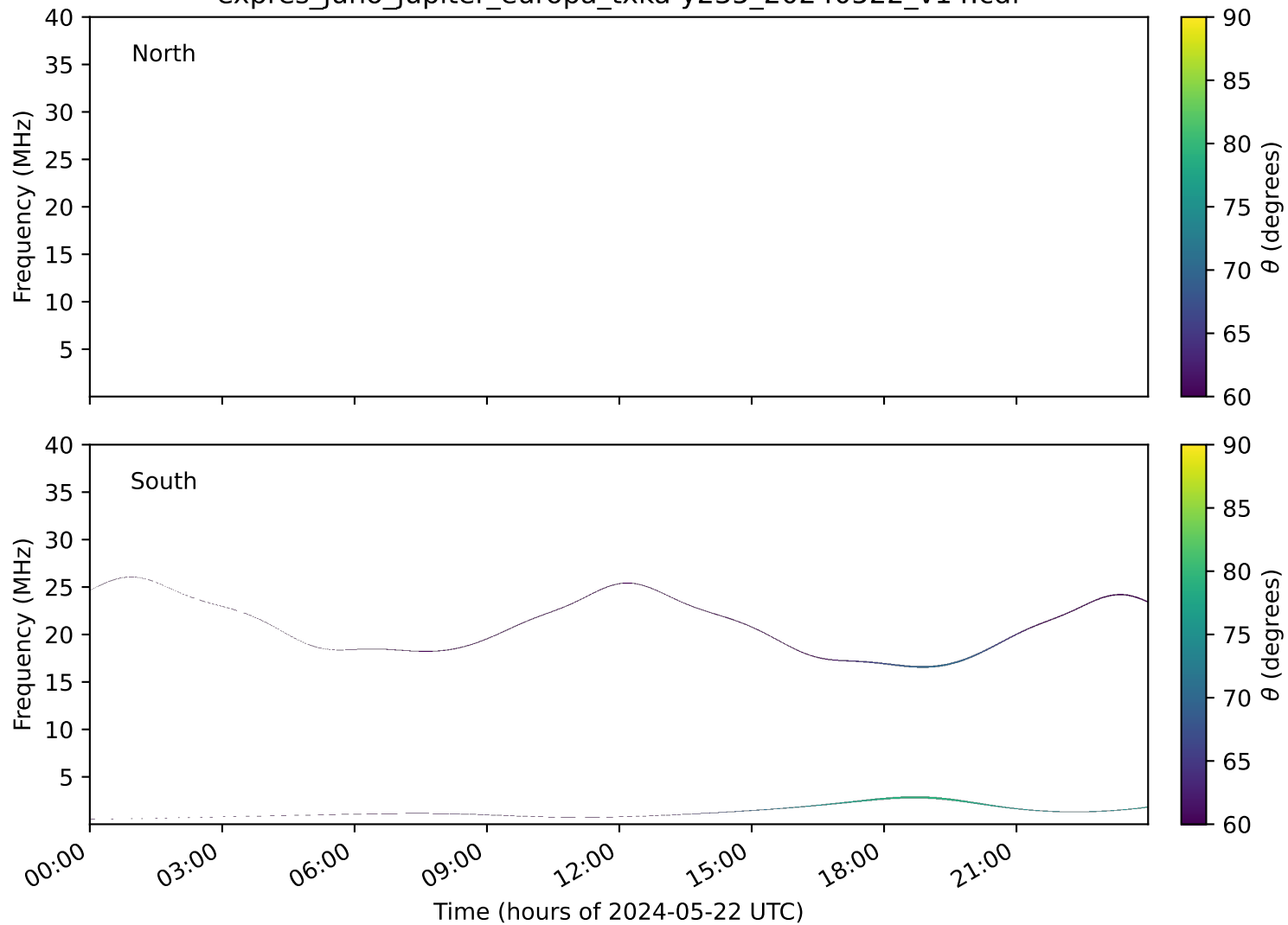
expres_juno_jupiter_europa_txka-y235_20240522_v14.cdf
