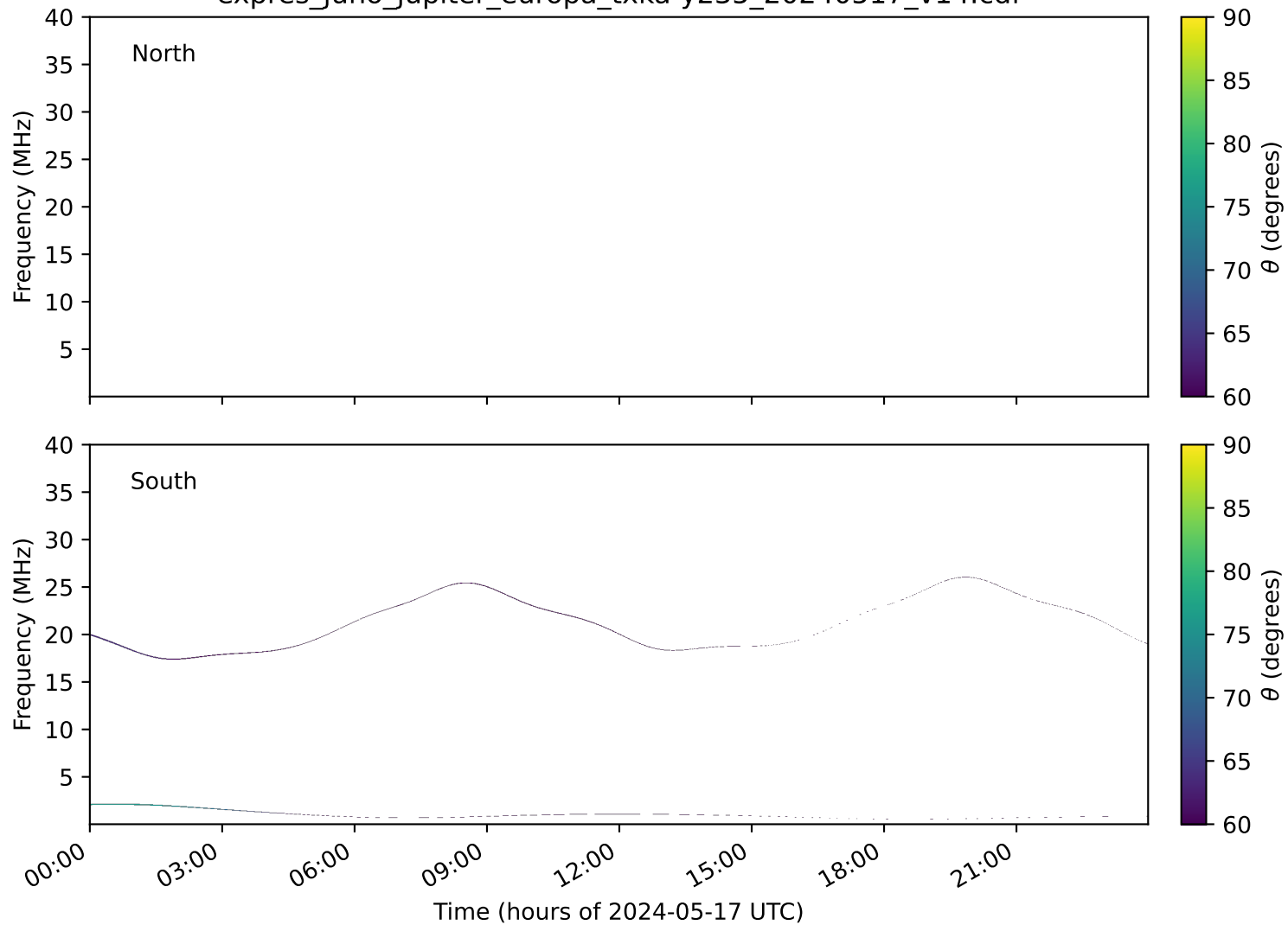
expres_juno_jupiter_europa_txka-y235_20240517_v14.cdf
