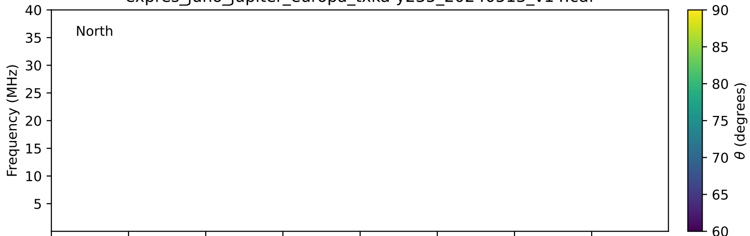
expres_juno_jupiter_europa_txka-y235_20240513_v14.cdf
