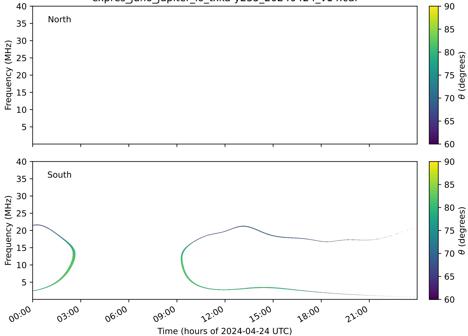
expres_juno_jupiter_io_txka-y235_20240424_v14.cdf
