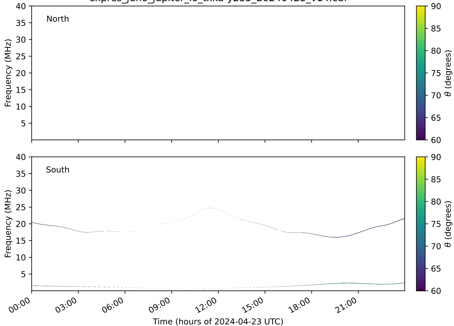
expres_juno_jupiter_io_txka-y235_20240423_v14.cdf
