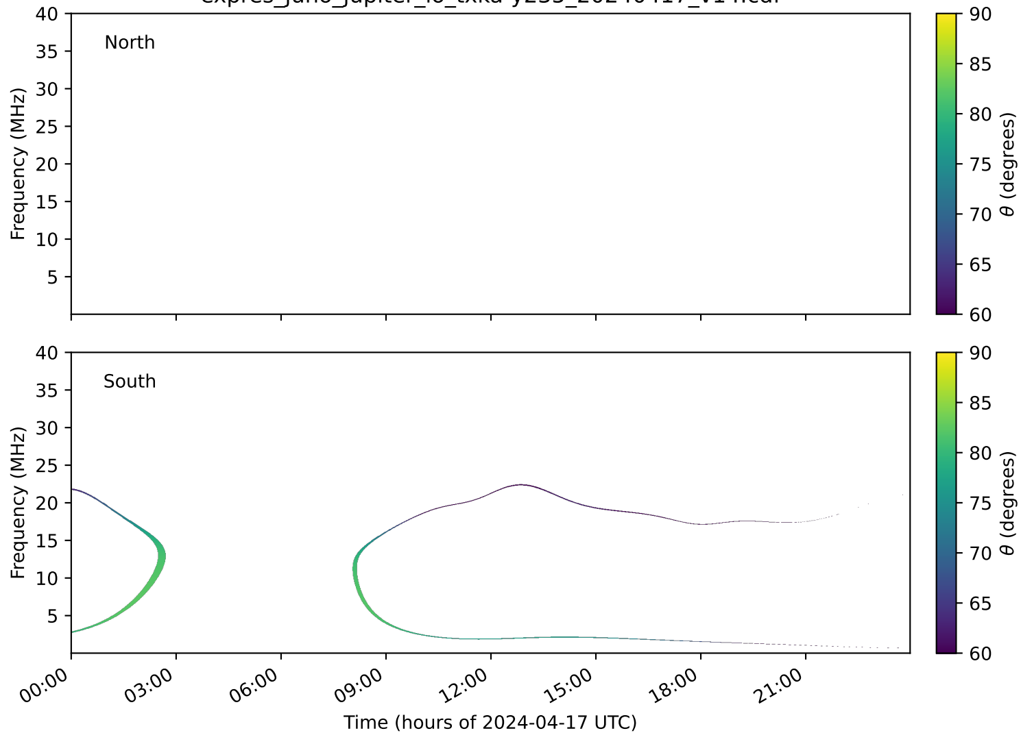
expres_juno_jupiter_io_txka-y235_20240417_v14.cdf
