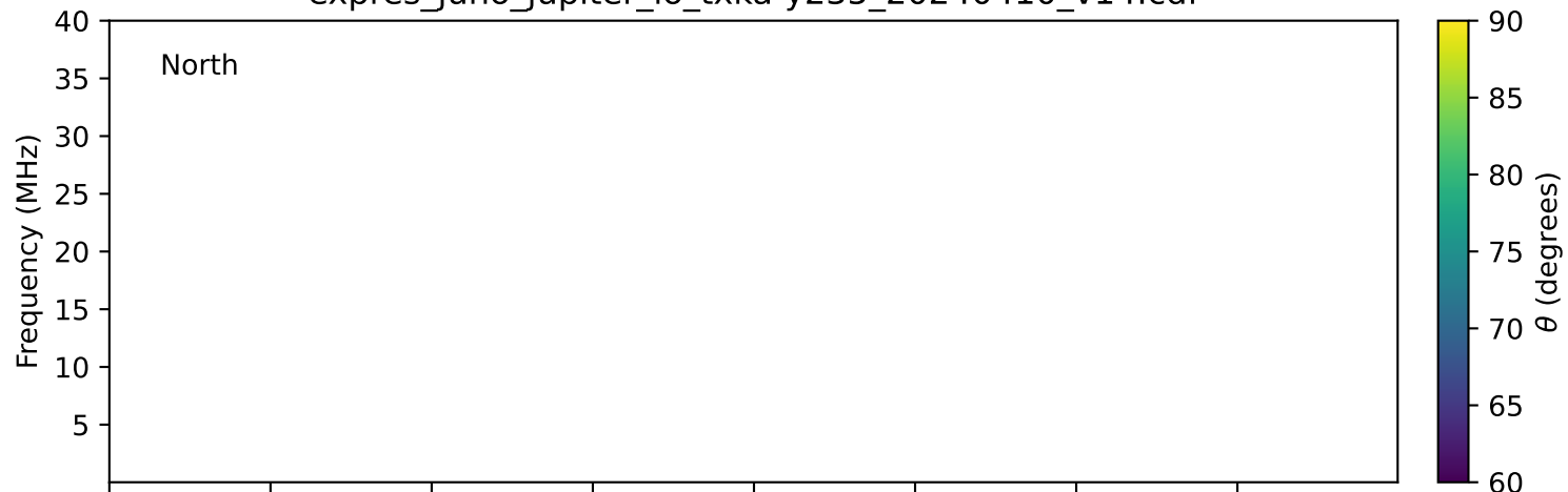
expres_juno_jupiter_io_txka-y235_20240410_v14.cdf
