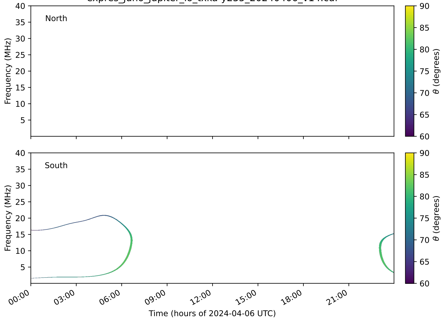
expres_juno_jupiter_io_txka-y235_20240406_v14.cdf
