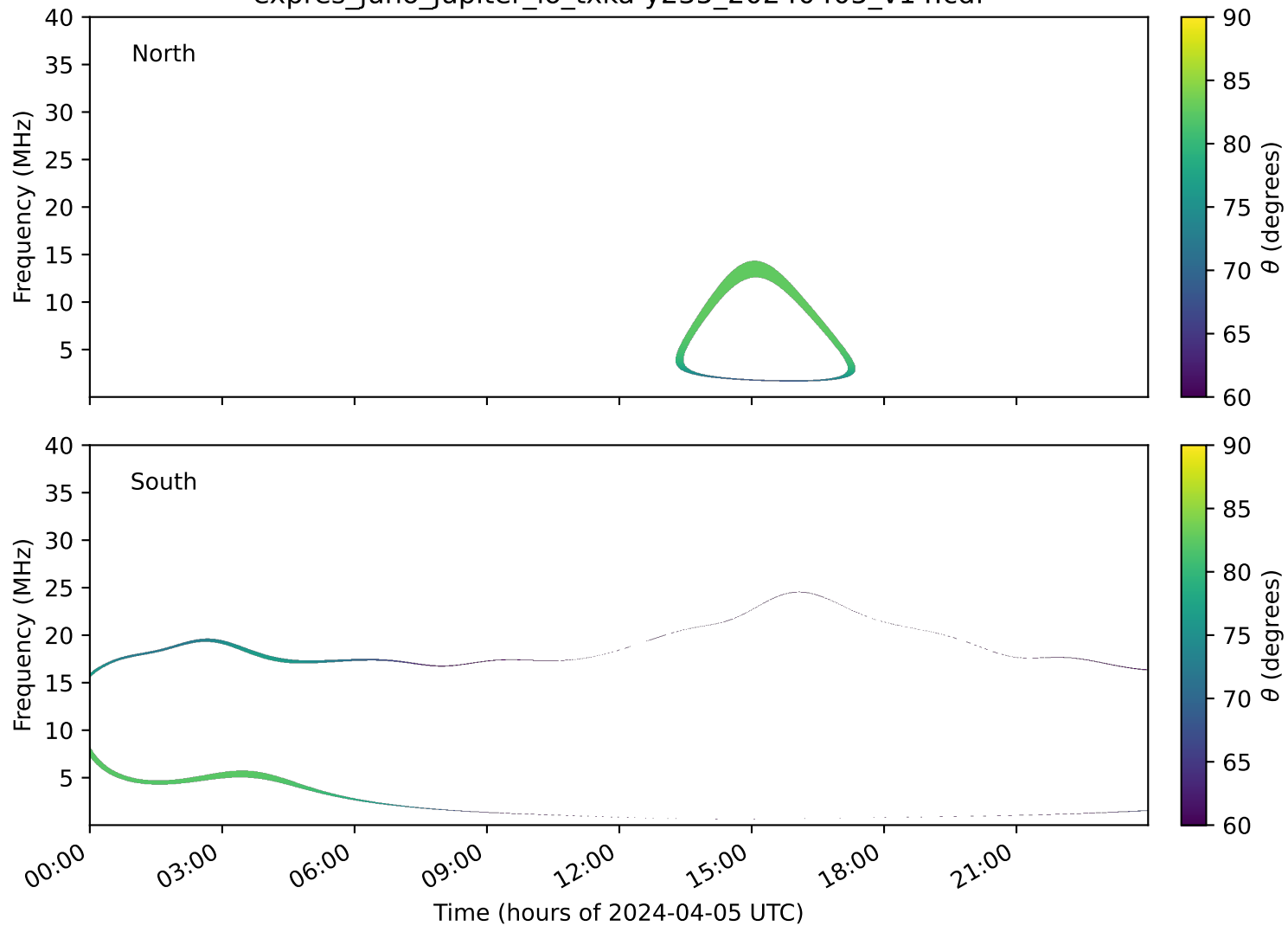
expres_juno_jupiter_io_txka-y235_20240405_v14.cdf
