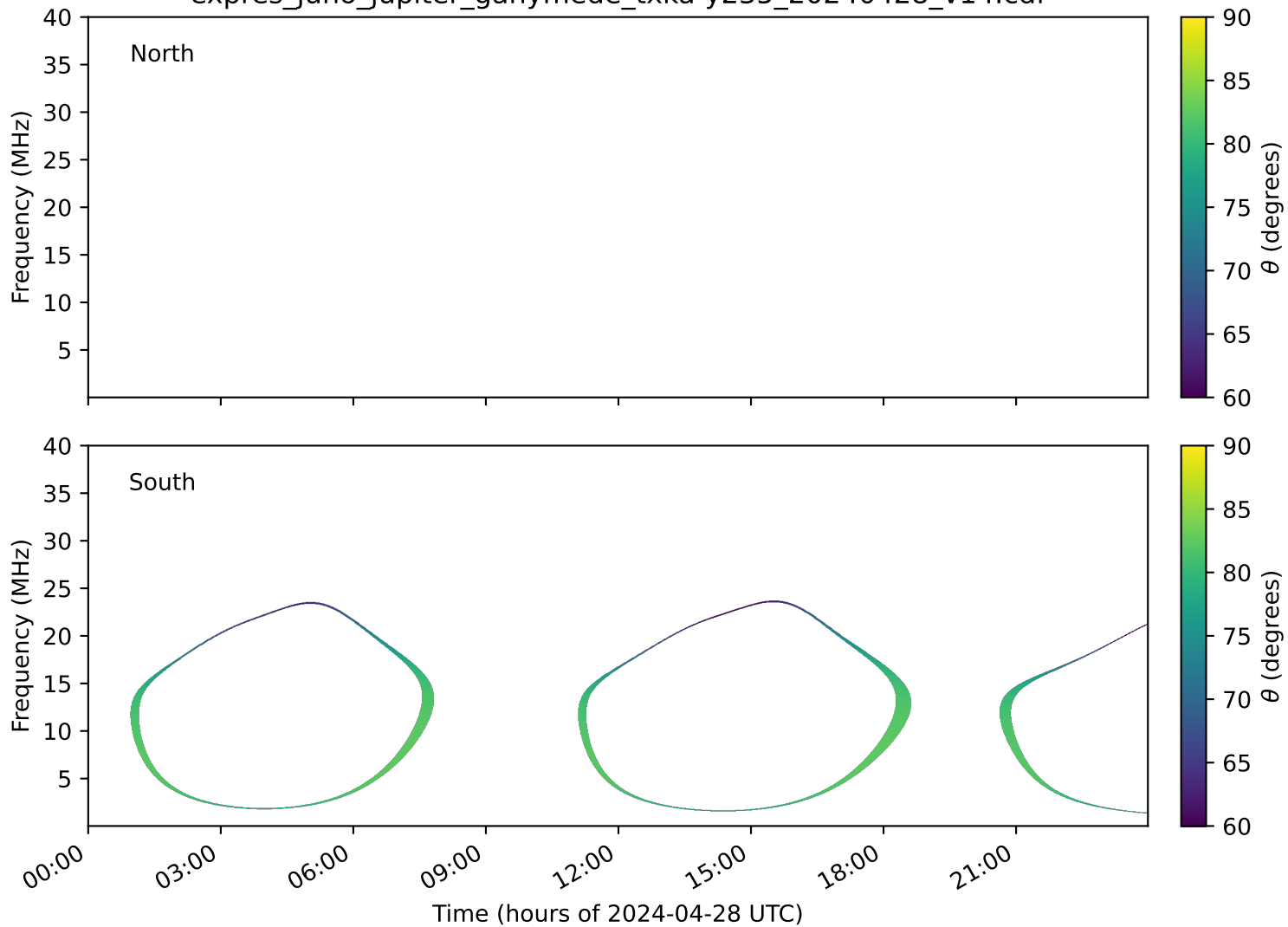
expres_juno_jupiter_ganymede_txka-y235_20240428_v14.cdf
