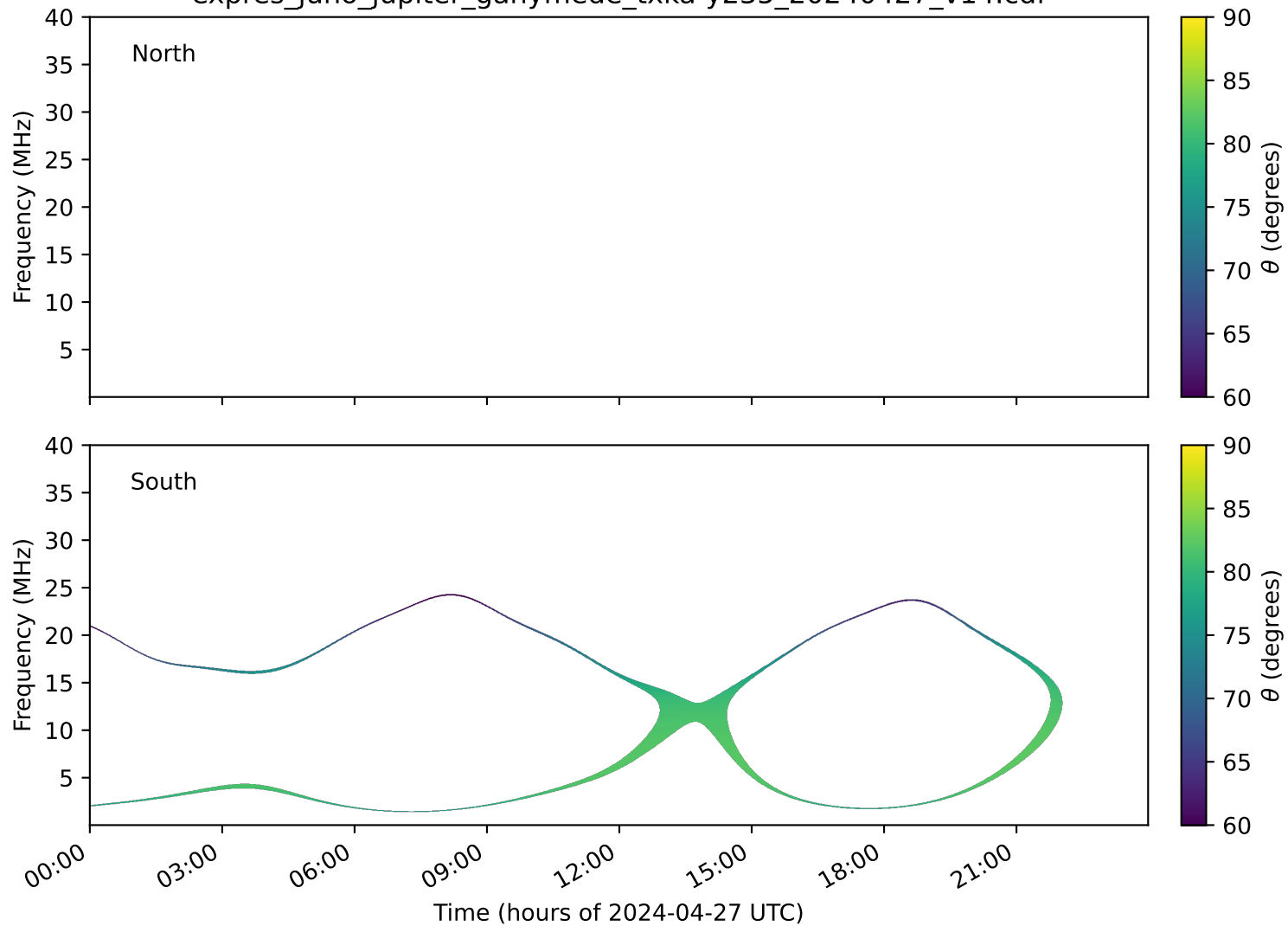
expres_juno_jupiter_ganymede_txka-y235_20240427_v14.cdf
