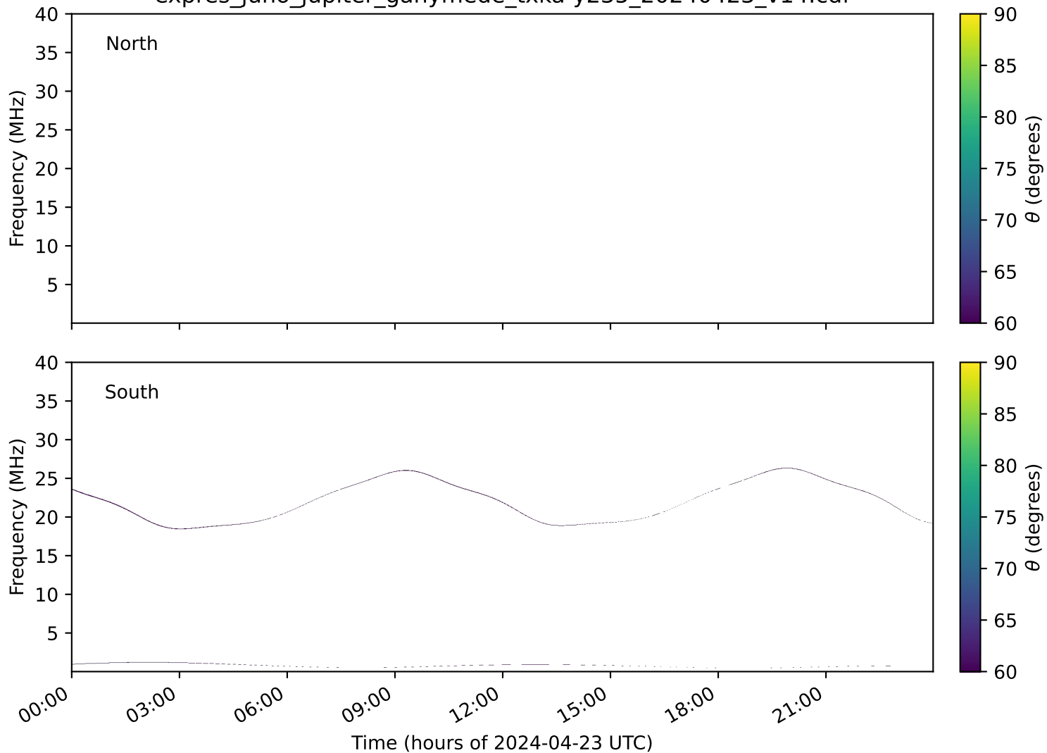
expres_juno_jupiter_ganymede_txka-y235_20240423_v14.cdf
