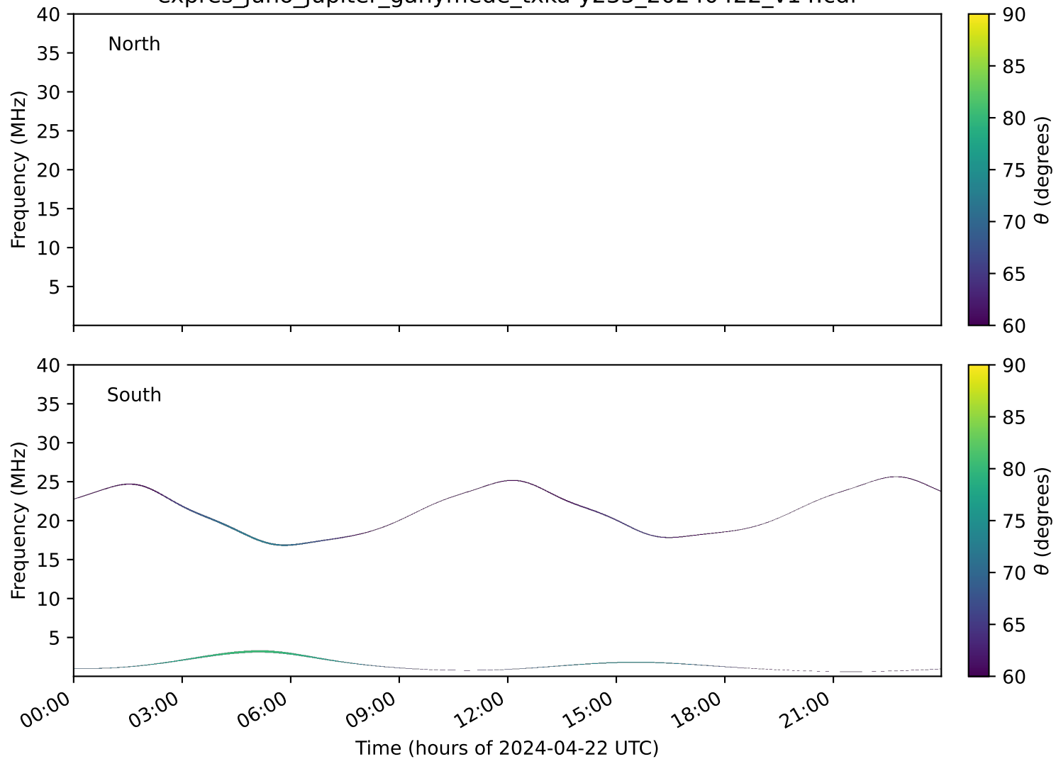
expres_juno_jupiter_ganymede_txka-y235_20240422_v14.cdf
