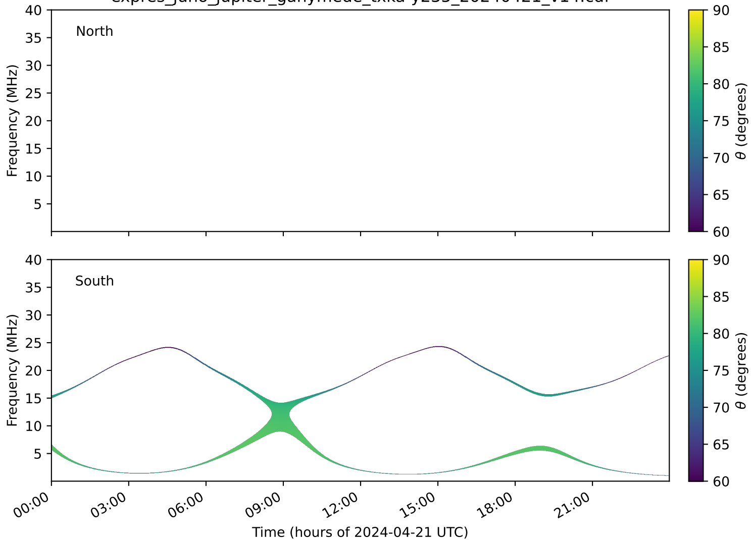
expres_juno_jupiter_ganymede_txka-y235_20240421_v14.cdf
