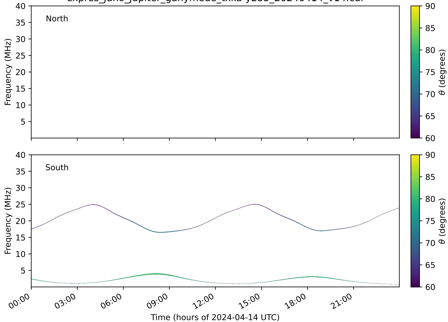
expres_juno_jupiter_ganymede_txka-y235_20240414_v14.cdf
