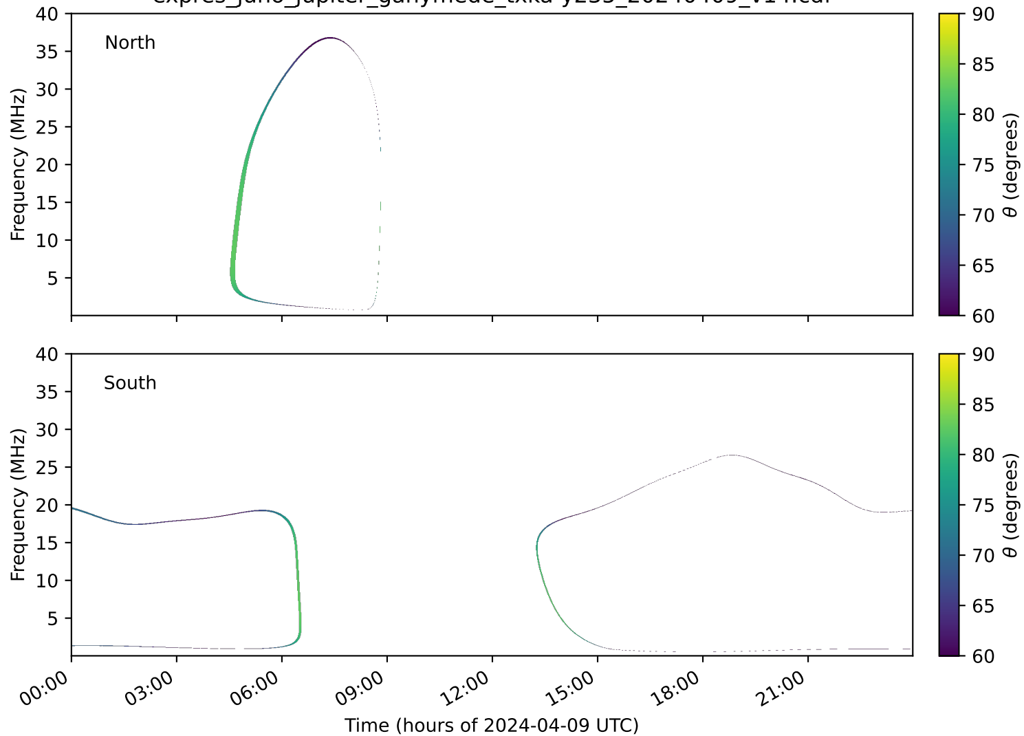
expres_juno_jupiter_ganymede_txka-y235_20240409_v14.cdf
