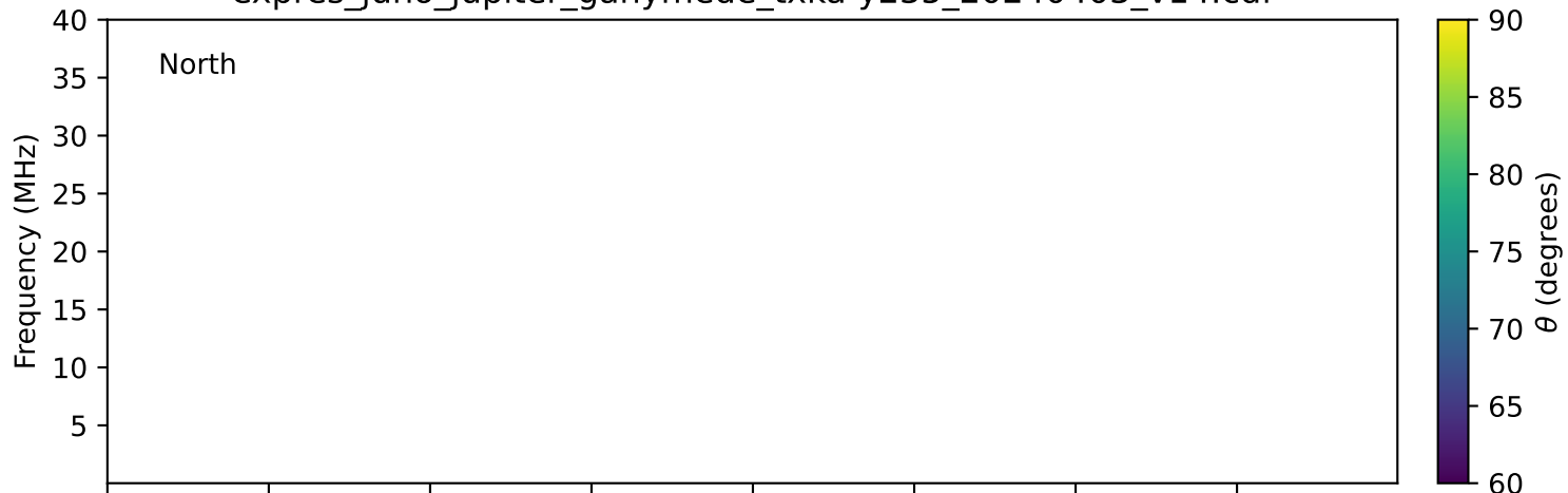
expres_juno_jupiter_ganymede_txka-y235_20240403_v14.cdf
