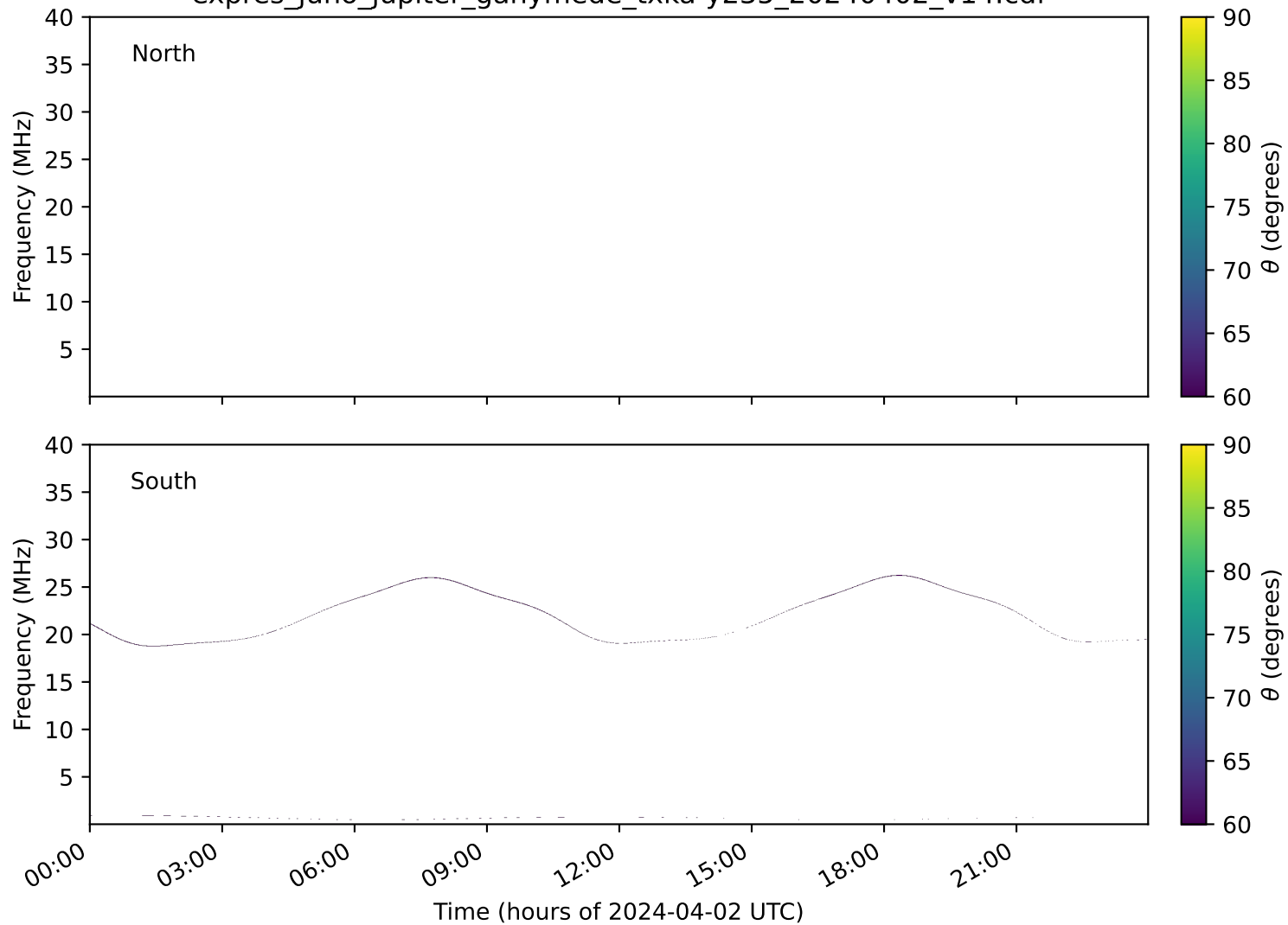
expres_juno_jupiter_ganymede_txka-y235_20240402_v14.cdf
