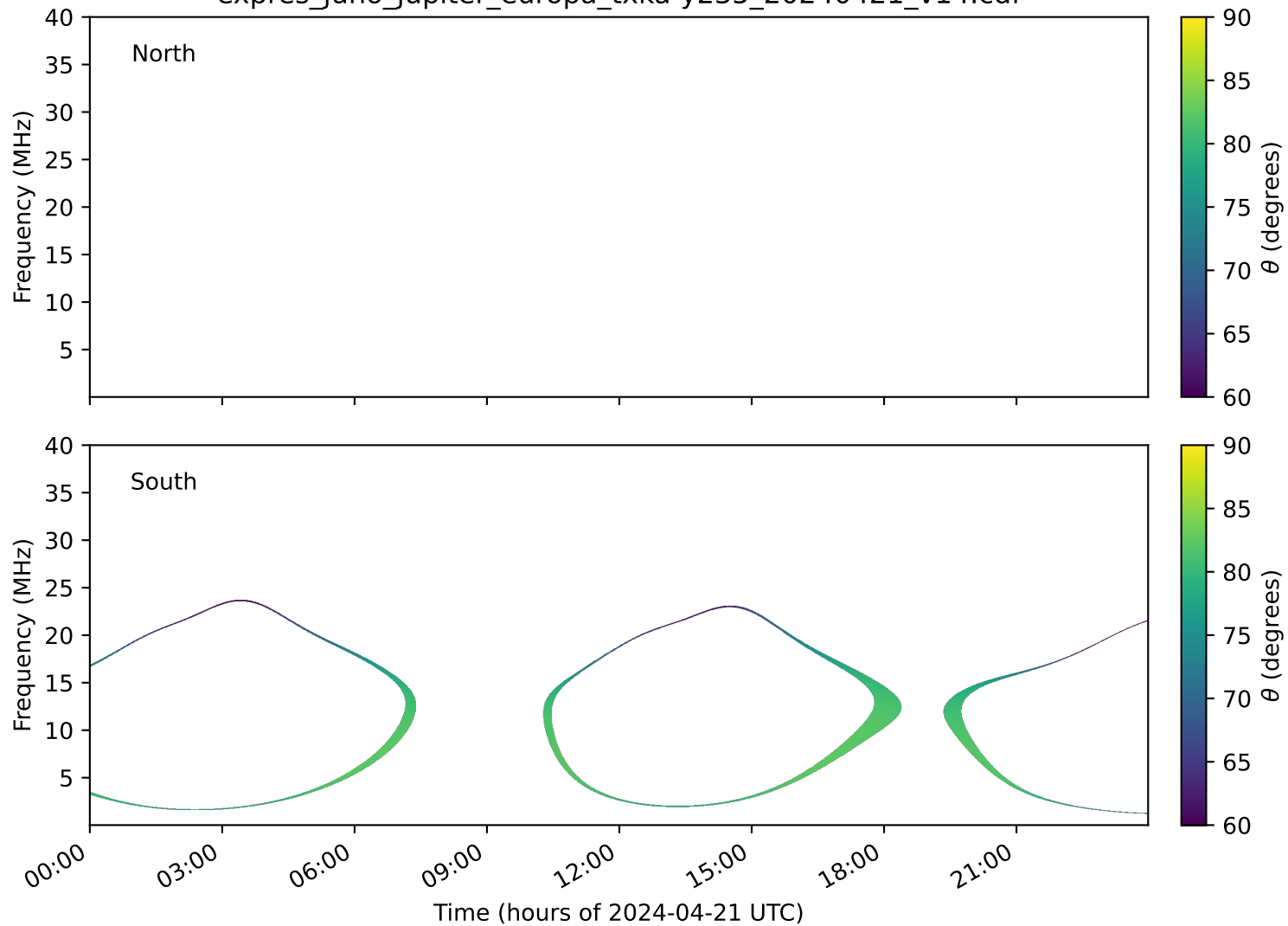
expres_juno_jupiter_europa_txka-y235_20240421_v14.cdf
