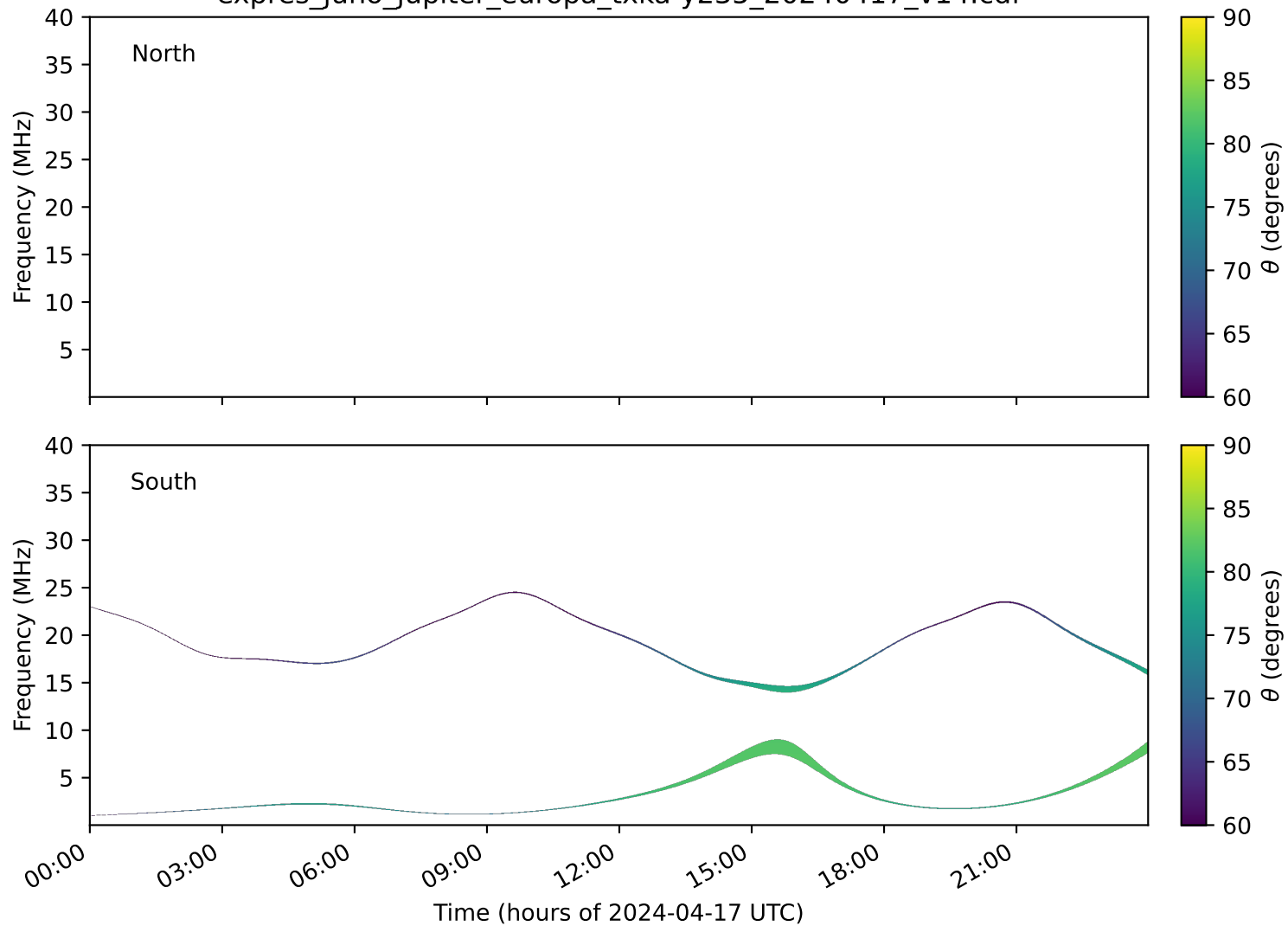
expres_juno_jupiter_europa_txka-y235_20240417_v14.cdf
