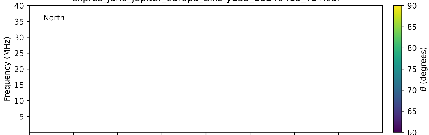
expres_juno_jupiter_europa_txka-y235_20240415_v14.cdf
