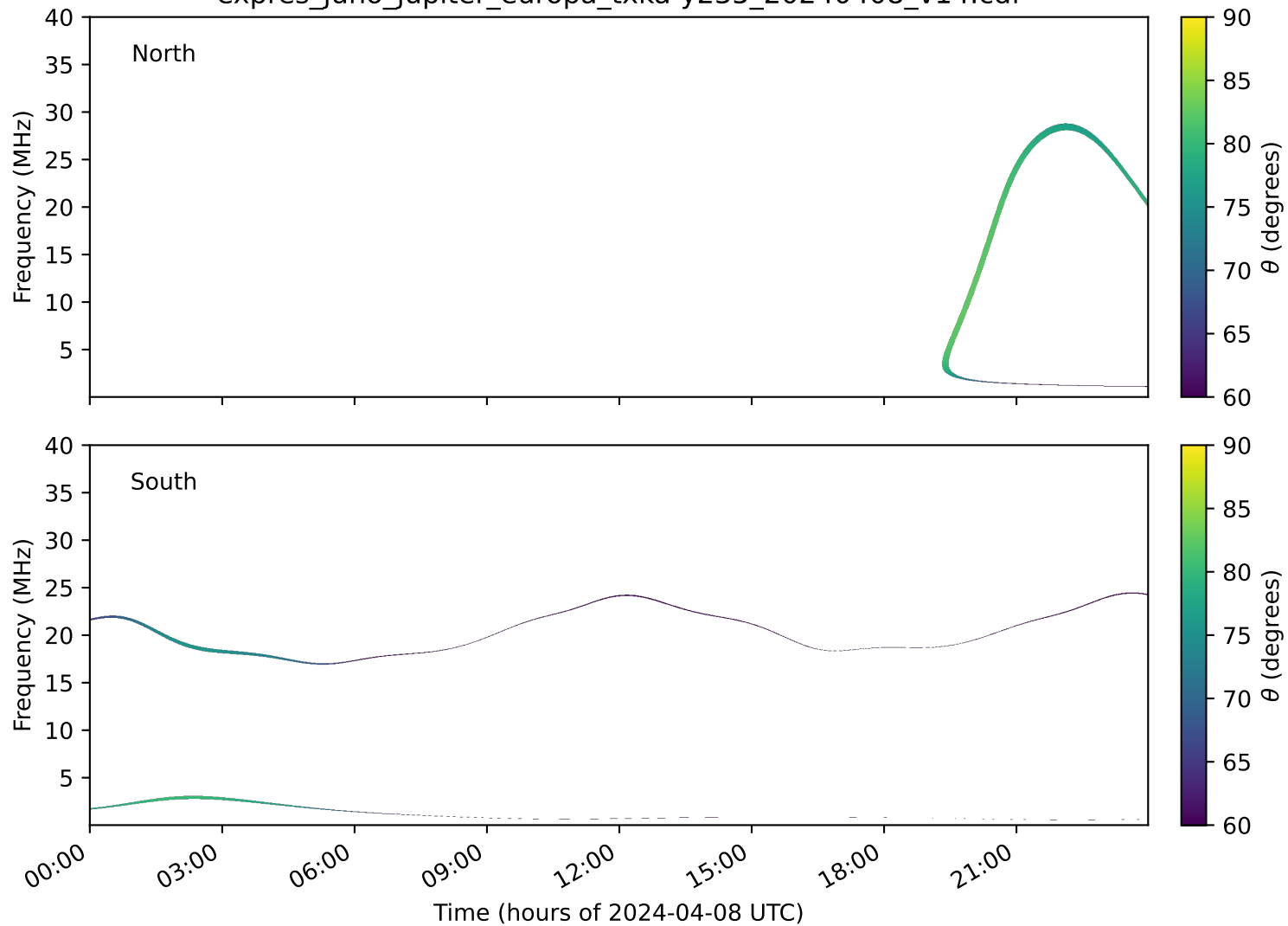
expres_juno_jupiter_europa_txka-y235_20240408_v14.cdf
