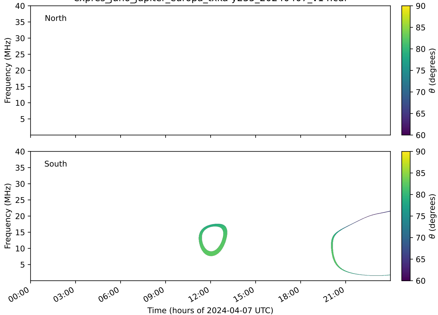
expres_juno_jupiter_europa_txka-y235_20240407_v14.cdf
