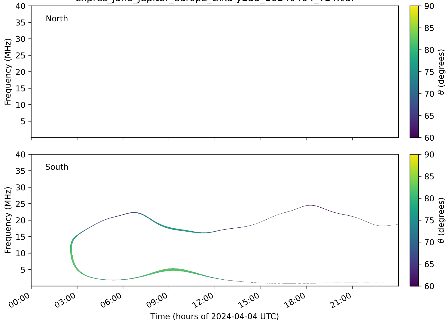
expres_juno_jupiter_europa_txka-y235_20240404_v14.cdf
