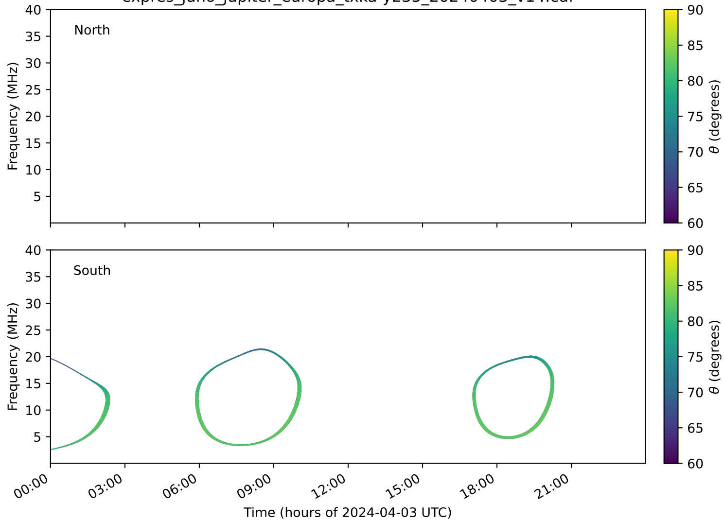
expres_juno_jupiter_europa_txka-y235_20240403_v14.cdf
