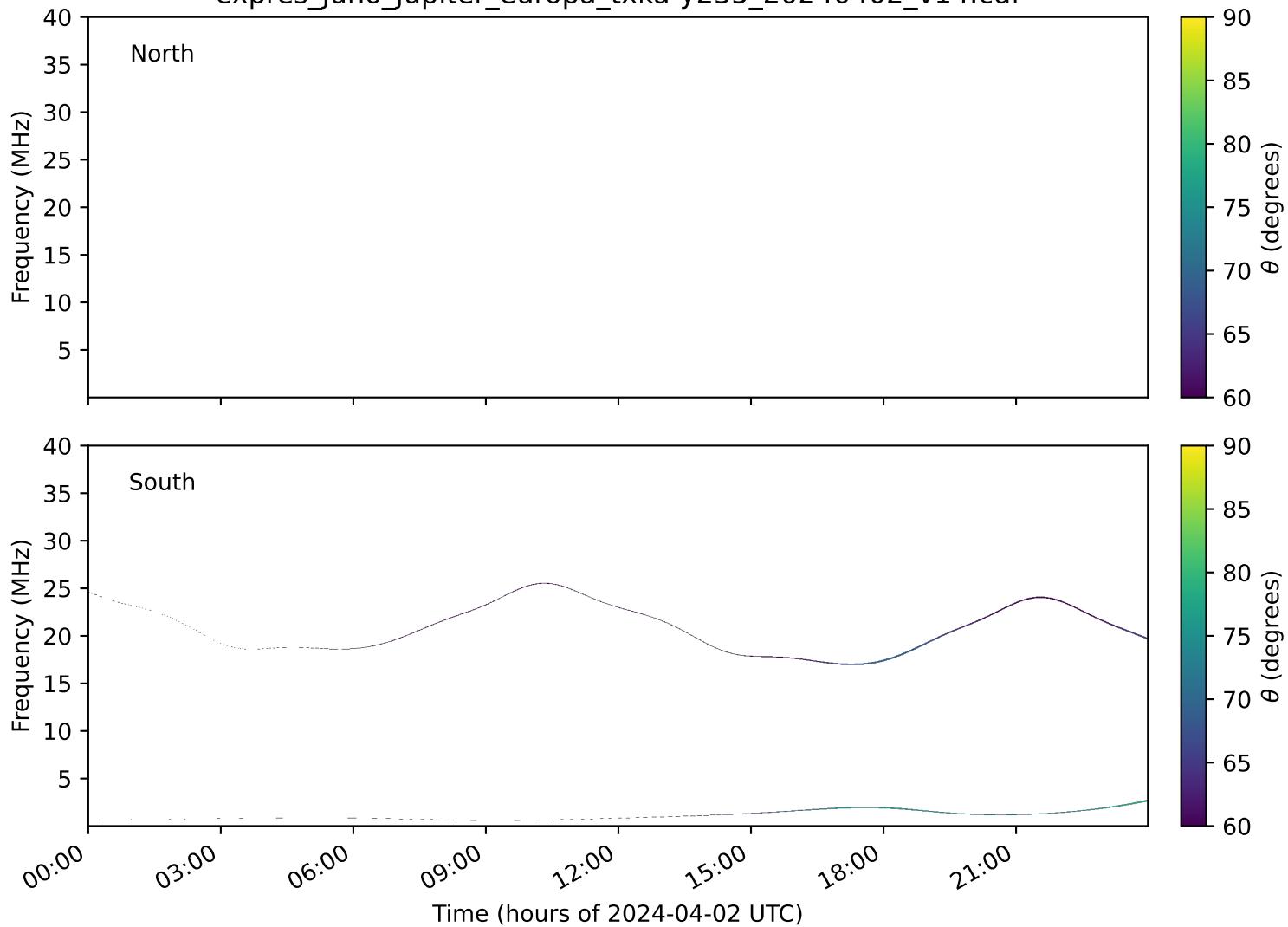
expres_juno_jupiter_europa_txka-y235_20240402_v14.cdf
