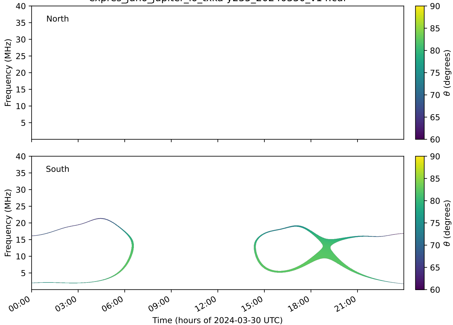
expres_juno_jupiter_io_txka-y235_20240330_v14.cdf
