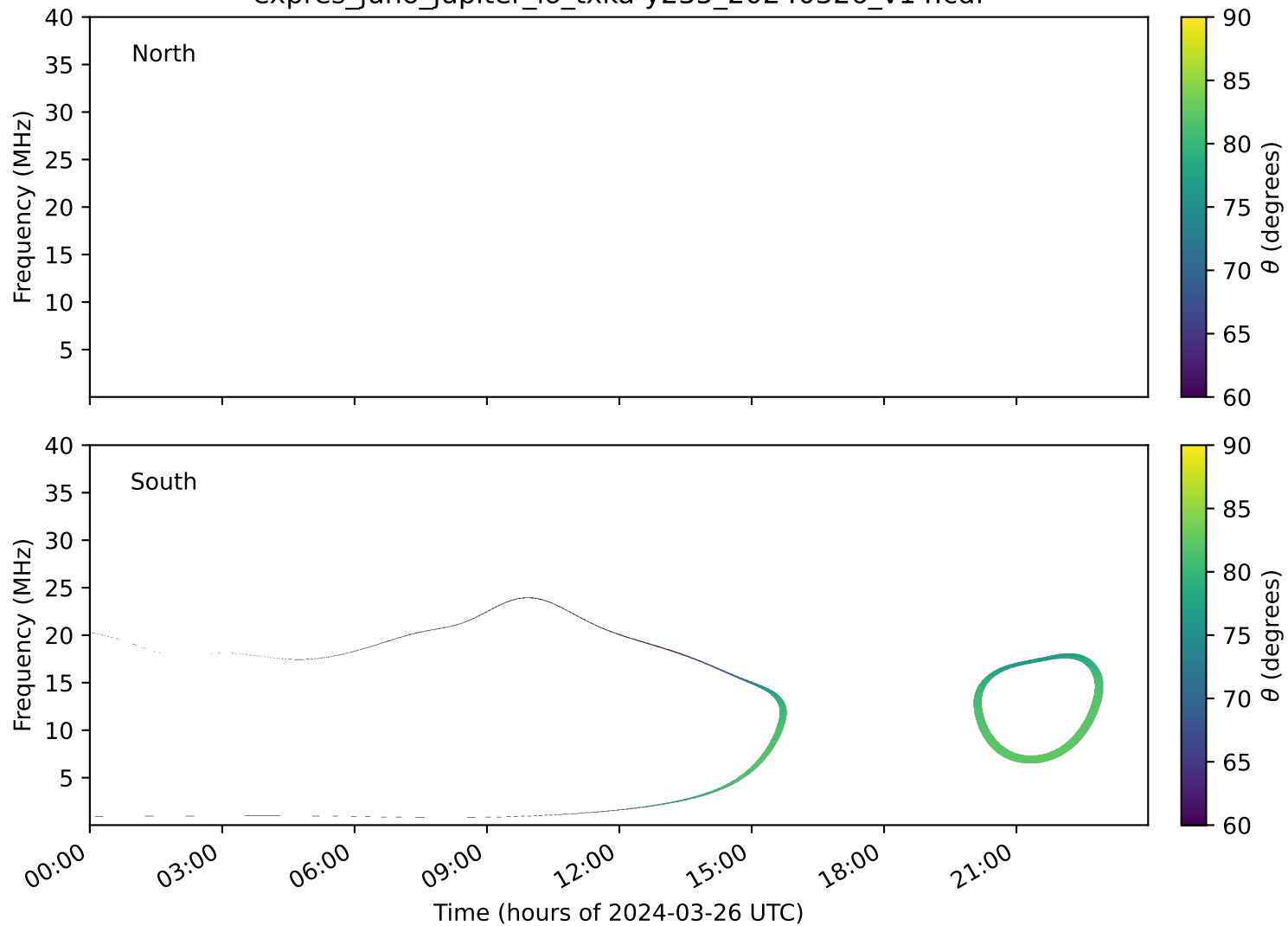
expres_juno_jupiter_io_txka-y235_20240326_v14.cdf
