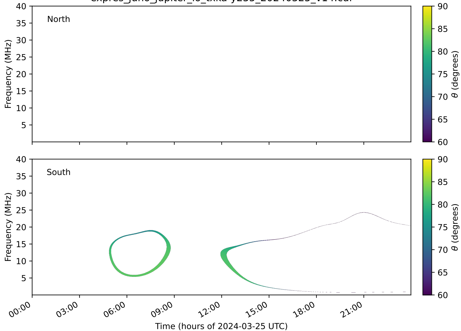
expres_juno_jupiter_io_txka-y235_20240325_v14.cdf
