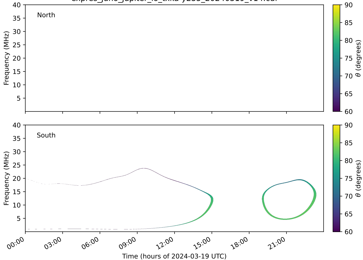
expres_juno_jupiter_io_txka-y235_20240319_v14.cdf
