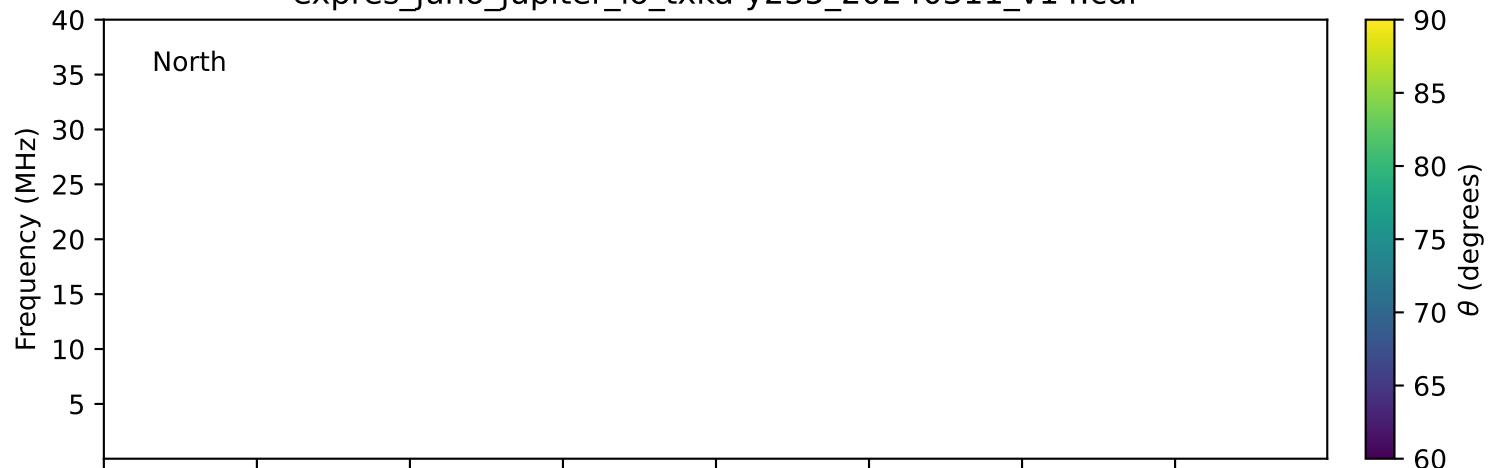
expres_juno_jupiter_io_txka-y235_20240311_v14.cdf
