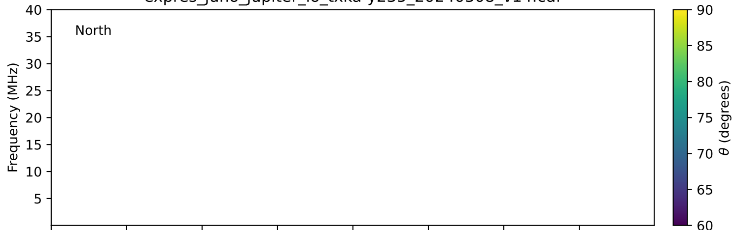
expres_juno_jupiter_io_txka-y235_20240308_v14.cdf
