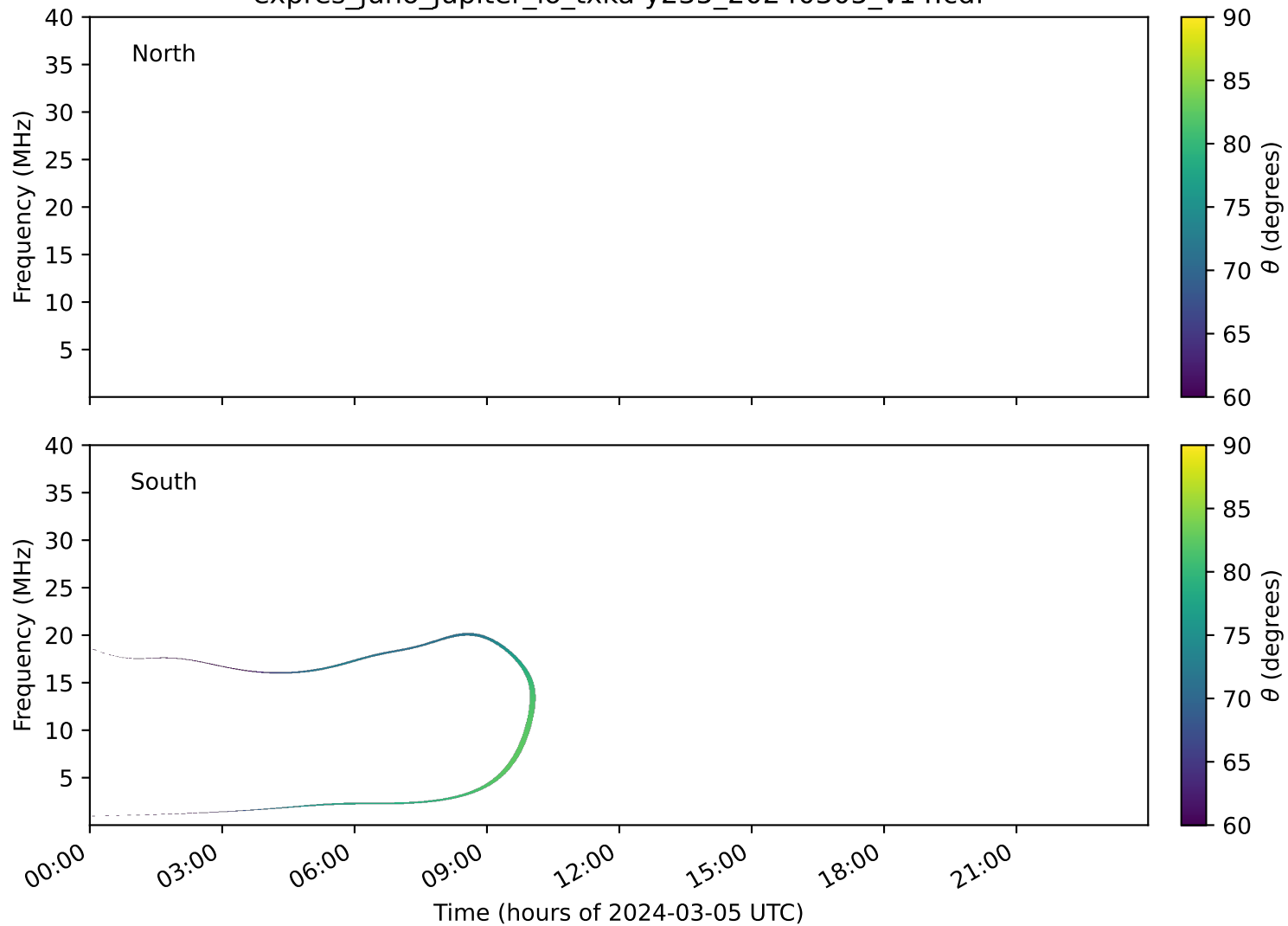
expres_juno_jupiter_io_txka-y235_20240305_v14.cdf
